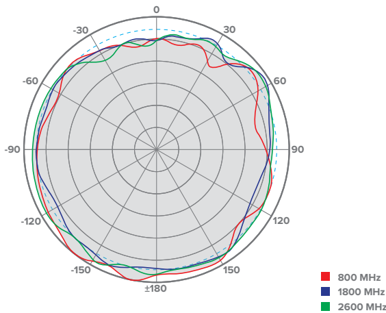
Elevation Radiation Pattern (Typical)
