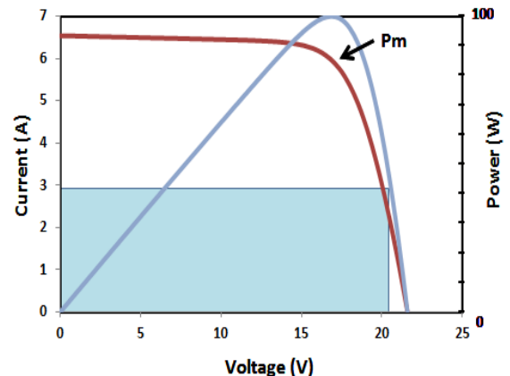
Fig 5: Less power harvested: voltage is too high
