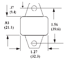
90° Bracket
