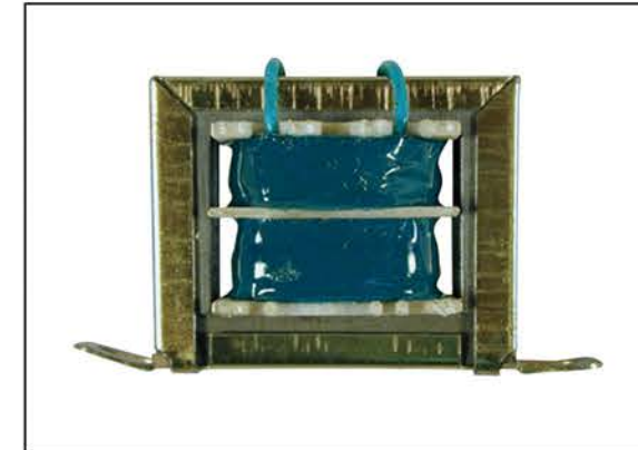
LP-360 (16V,120ma) LP-421 (6-0-6V, 0.3A) LP-423 (9-0-9V, 0.5A) LP-426 (6-0-6V, 0.5A) LP-427 (6-0-6V, 1A) LP-428 (6-0-6V, 2.A) LP-430 (6-0-6V, 4A) LP-433 (9-0-9V, 1A) LP-435 (9-0-9V, 1.5A) LP-437 (9-0-9V, 2A) TRANSFORMERS • Universal • Center Taps • 110V/220V • 9-0-9V, 2A
