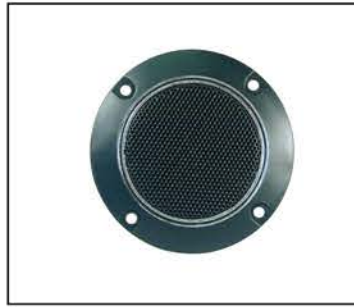
NTX-1006PZG ROUND PIEZO TWEETER W/ GRILL • Frequency Range: 2K~20KHz • Power RMS/Max: 75/150W • Impedance: 4-8 Ohms • Mounting Diameter: 66mm
