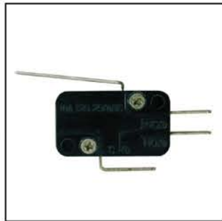
EC-284 SPDT ON-ON MICRO SWITCH • Current Rating: 10A 125V AC • 2 Pins
