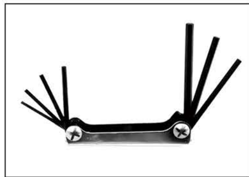
IHKS-307 FOLDING HEX KEY SET • 7 Piece Folding Hex Key Set • 1/16", 5/64", 3/32", 1/8", 5/32", 3/16", 7/32" Sizes
