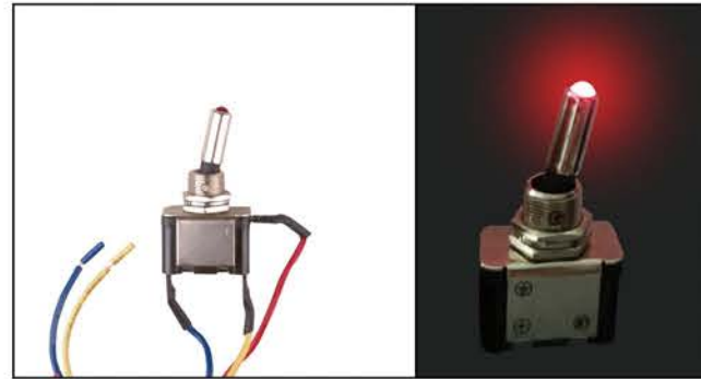
IS-EC-MT1220RED MATEL TOGGLE SWITCH WITH RED COLOR LED AND 6" LEAD WIRE • Current Rating: 20A, 12V • 2 Pins
