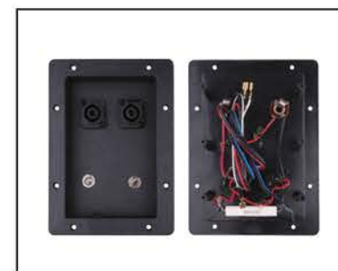
X-870 2 SPKN • 2 1/4" Sockets • 7" x 5" • With Crossover
