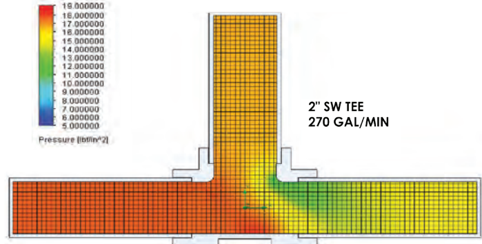
MEP995SBW-16 vs. standard tee
