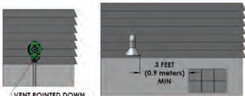
Figure 2: Regulator with Vent Pointed Down
