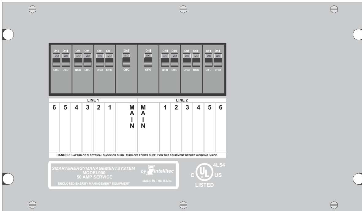
50 Amp EMS Distribution Panel P/N 00-00894-600
