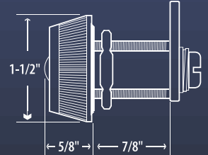
3/4" Cylinder Nut
