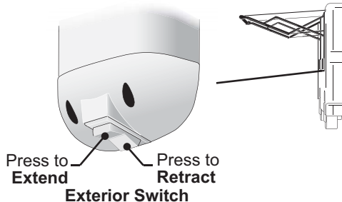
Exterior Switch
