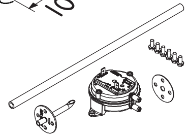
Pressure Switch Kit Included with MD6TU, MD8TU & MD10TU
