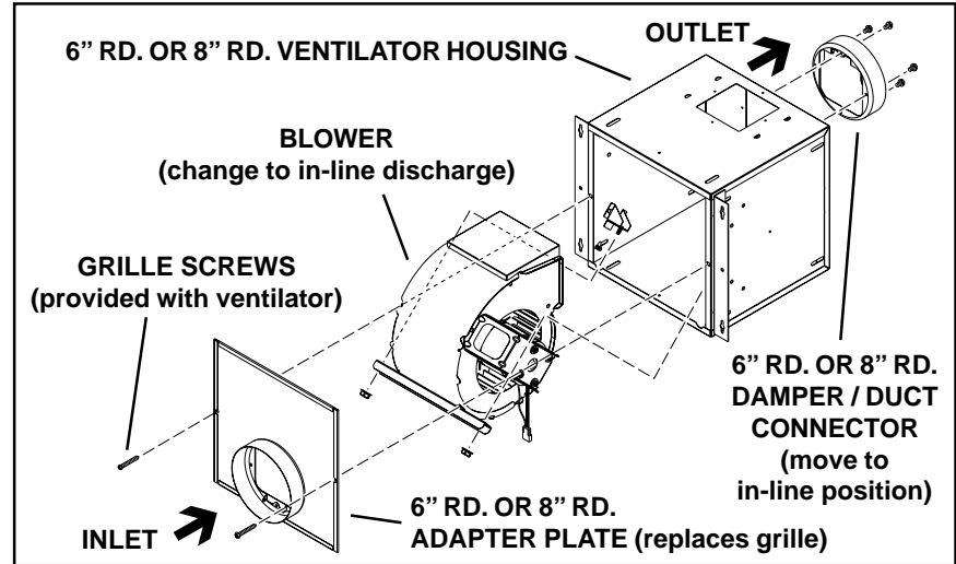
6" ROUND & 8" ROUND VENTILATOR Straight-Through Discharge
