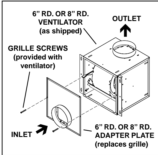
6" ROUND & 8" ROUND VENTILATOR Right Angle Discharge
