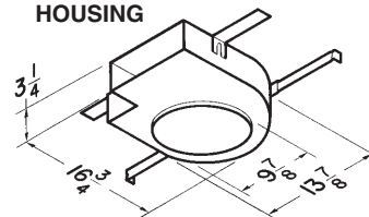
MODEL 502 HOUSING
